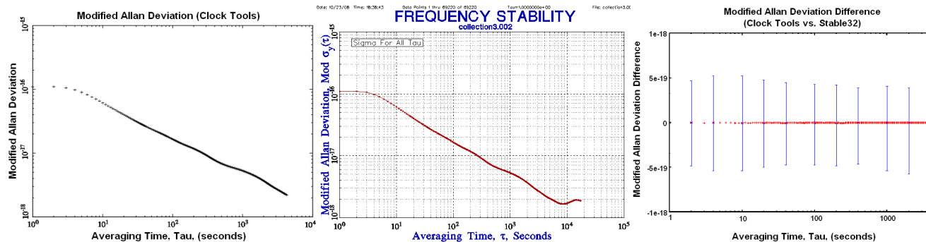
Figure 3: Modified Allan Deviation Comparison a) Clock Tools Implementation, b) Stable32 Implementation, c) Difference Plot
