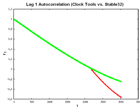
Figure 15: Autocorrelation Comparison
