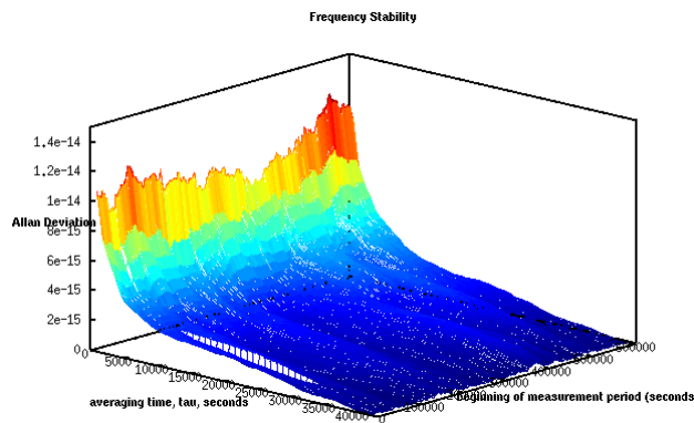
Figure 6: A Dynamic Allan deviation plot
