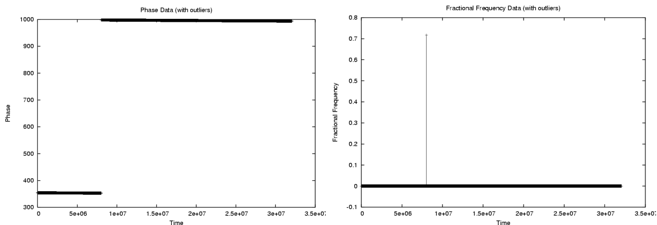
Figure 7: Conversion from Phase to Fractional Frequency a) Phase data with a phase jump, b) Data represented as fractional frequency
