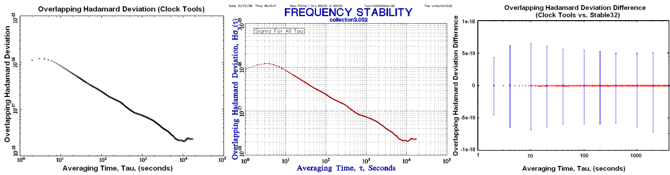
Figure 5: Overlapping Hadamard Deviation Comparison a) Clock Tools Implementation, b) Stable32 Implementation, c) Difference Plot
