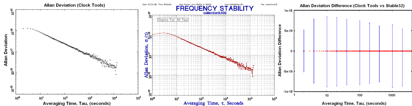
Figure 1: Allan Deviation Comparison a) Clock Tools Implementation, b) Stable32 Implementation, c) Difference Plot
