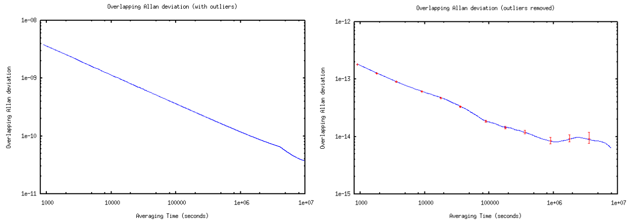
Figure 9: Overlapping Allan deviations
