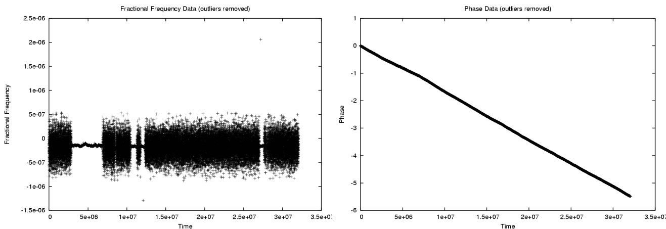
Figure 8: Conversion from Fractional Frequency to Phase a) Fractional frequency data with spike removed, b) Phase data with phase jump removed
