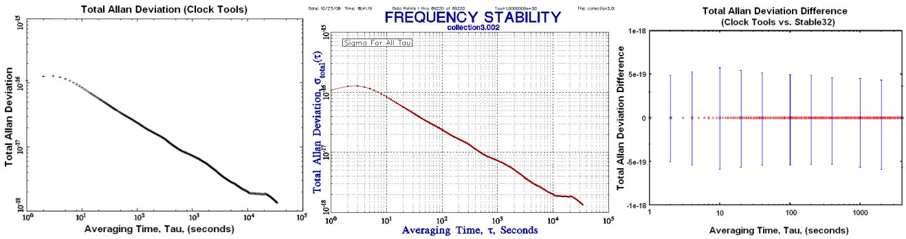
Figure 4: Total Allan Deviation Comparison a) Clock Tools Implementation, b) Stable32 Implementation, c) Difference Plot
