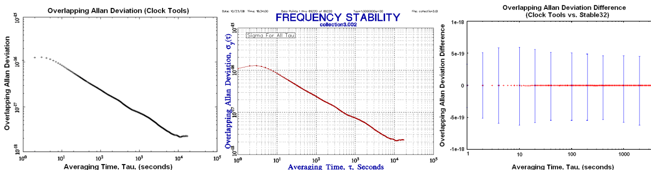
Figure 2: Overlapping Allan Deviation Comparison a) Clock Tools Implementation, b) Stable32 Implementation, c) Difference Plot
